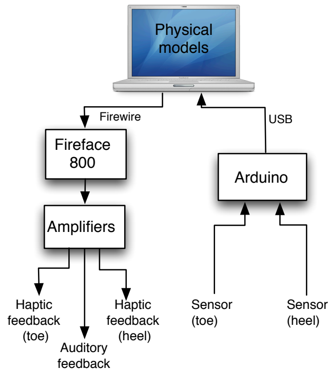
Fig. 1. Diagram illustrating the different hardware components of the system, together with their connections to the PC. The representation is for one shoe.
